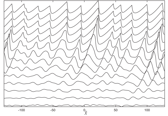
Fig. 16. Decelerated case with (26) \bar{l}_s = 1 . Spatio-temporal diagram, time increases from bottom to top. There is a final steady bed because the shear stress is under the threshold.
