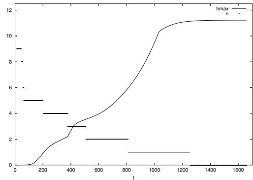
Fig. 10. Steady case \bar{U}'_S = 1 , \tilde{l}_s = 1 , evolution of the maximum value and of the number of bumps in the domain versus time.
